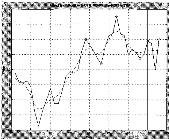
(a) Head-and-Shoulders
